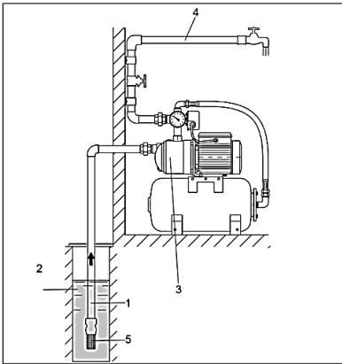
Installation of water pump – well
