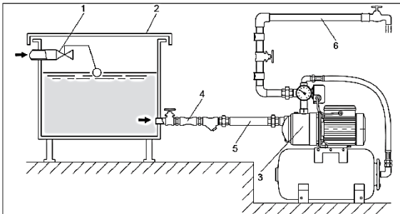
Hydrophore assembly - buffer vessel
